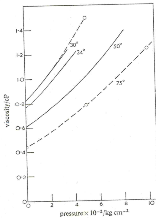
FIG. 7.—The viscosity of cyclohexane. ○, Bridgman 7 ; —, this work.
