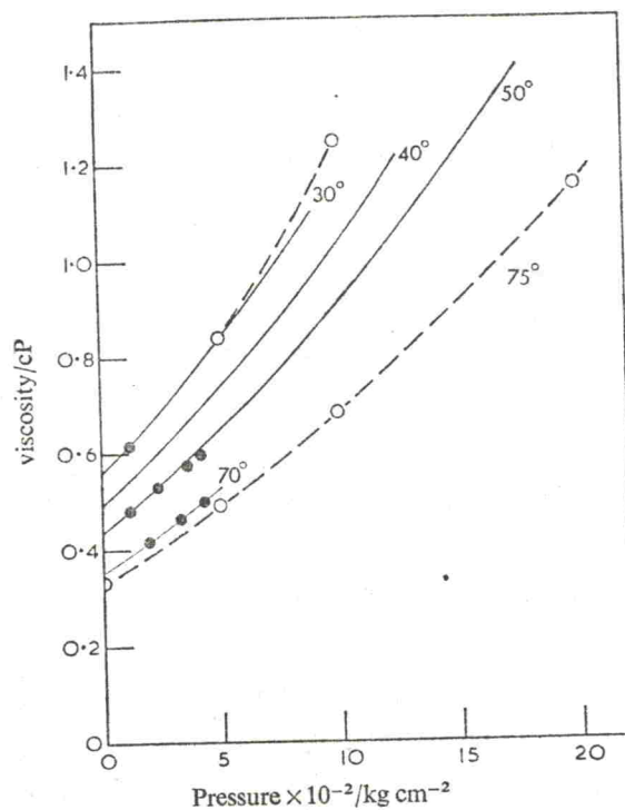
FIG. 6.—The viscosity of benzene. ●, Jobling and Lawrence; ○, Bridgman 7 ; —, this work.
